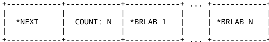
__BRANCH_TABLE__ layout
